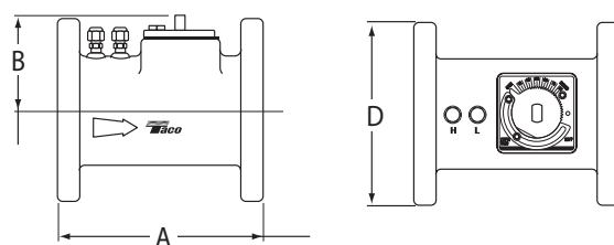
2-1/2", 3", 4" FLANGED
