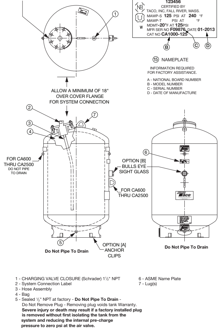
DIAGRAM 1 – LOCATION OF TANK FITTINGS
