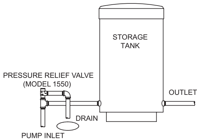
TYPICAL INSTALLATION
